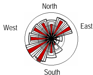
Figure 4 - Wind rose
