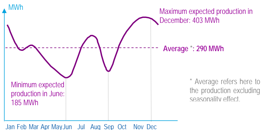
Figure 9 - La Venta III, Net Monthly production per turbine
