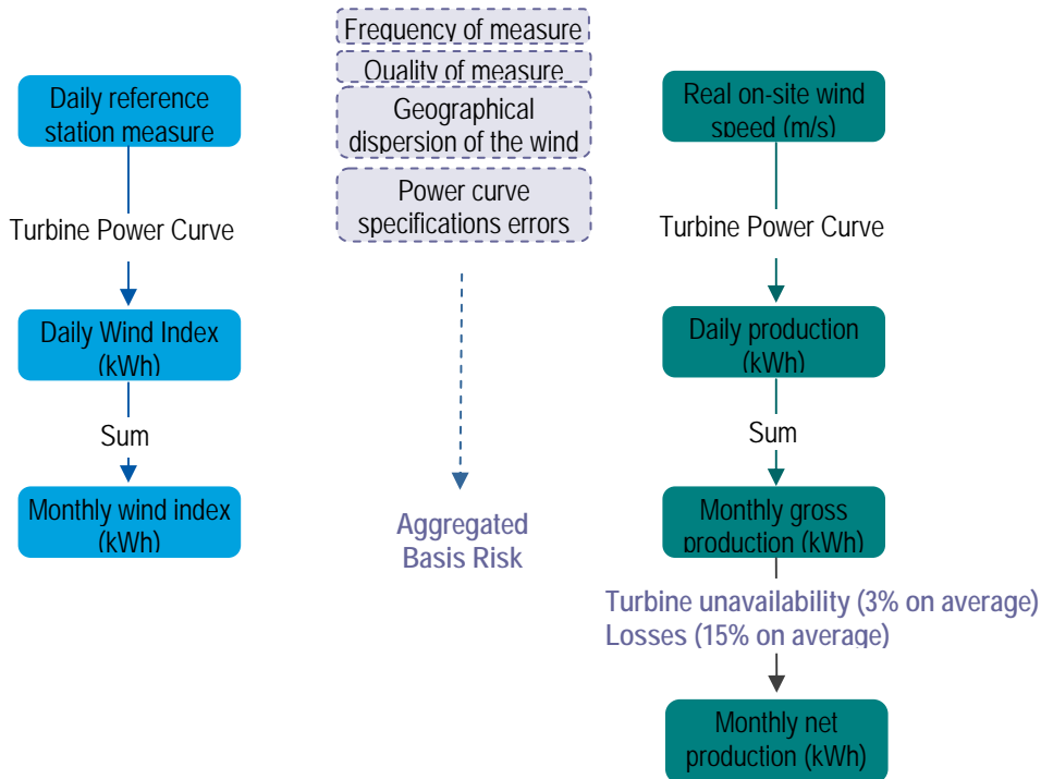
Figure 18 - Wind Index Construction
