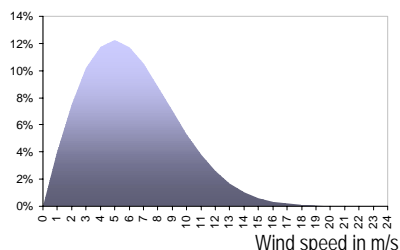
Figure 3 - Wind speed distribution probability
