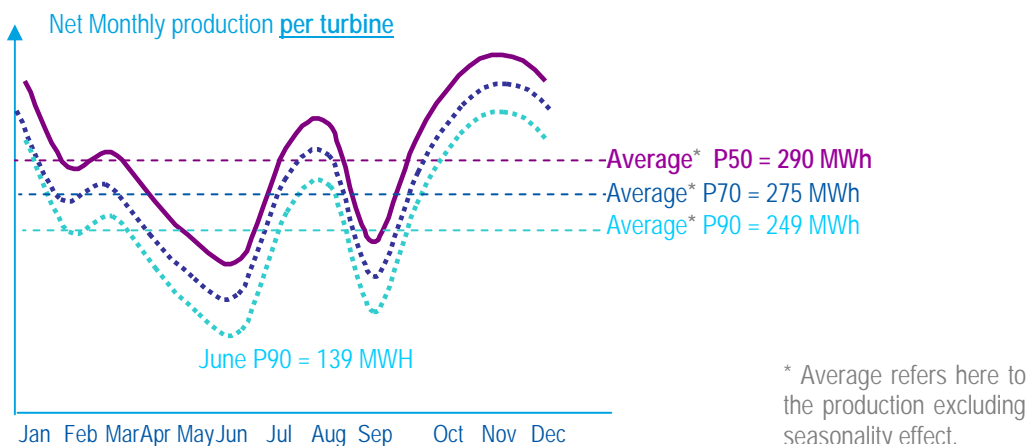
Figure 10 – La Venta III, Net monthly production per turbine with exceedance probabilities
