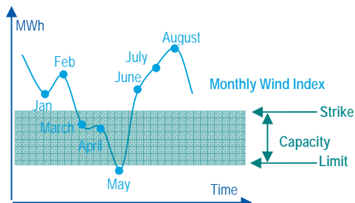
Figure 1 - Monthly wind derivative mechanism
