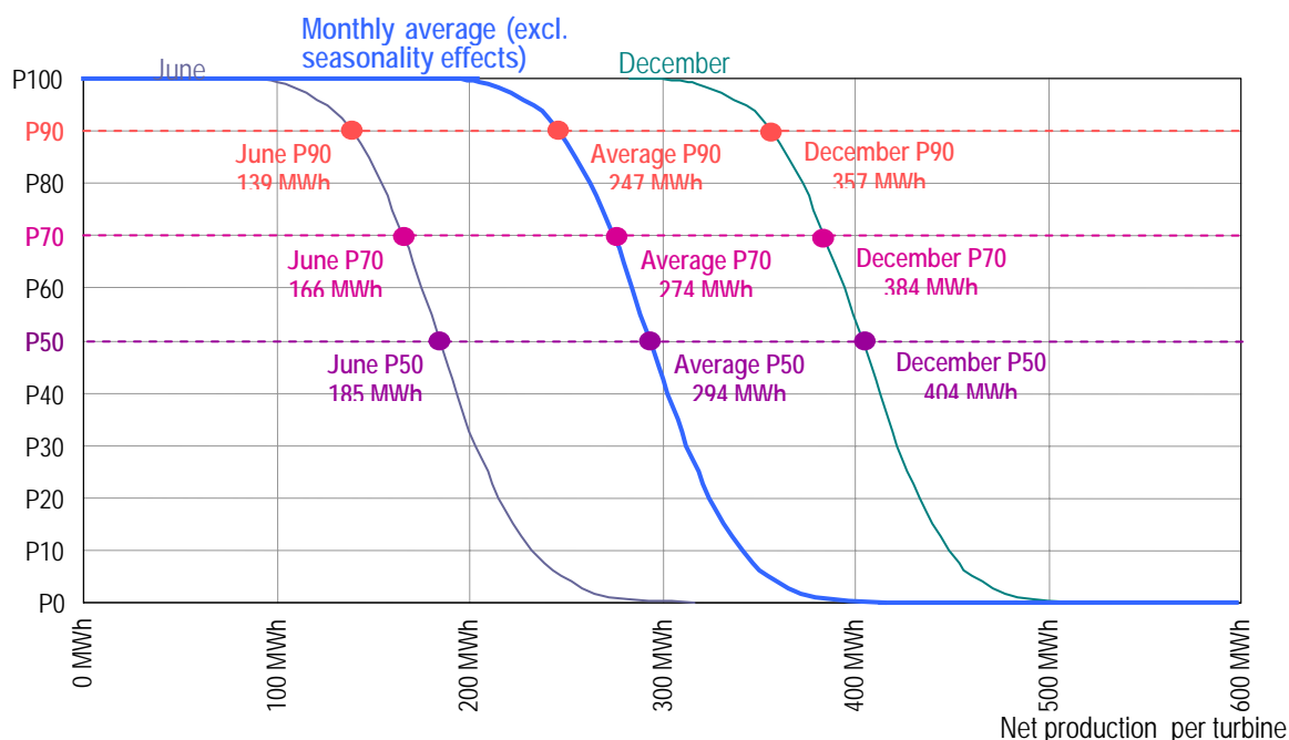
Figure 11 - La Venta III; Probability curves of Net production per turbine
