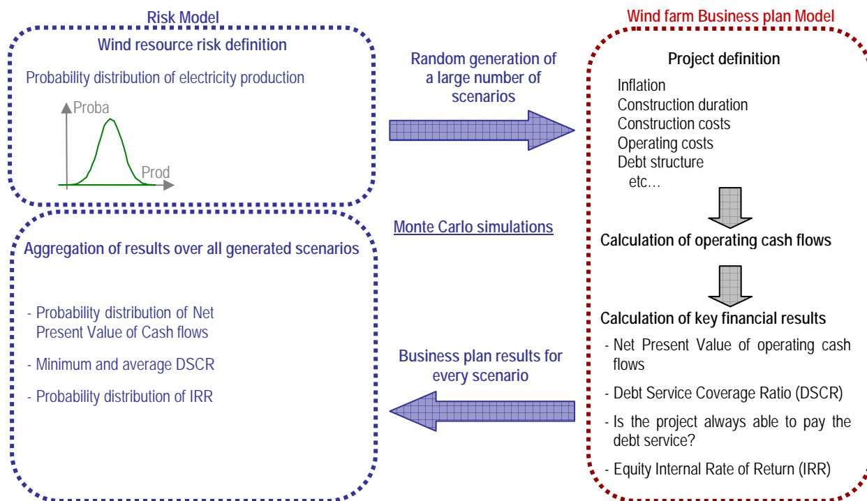
Figure 20 - Wind farm stochastic business plan model
